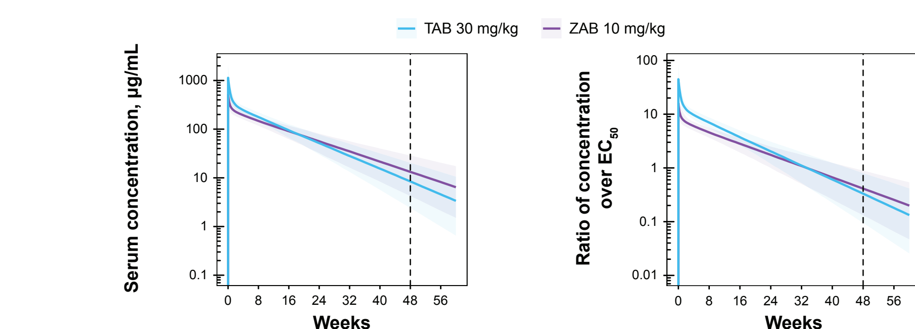
Figure 7. Simulated bNAB serum concentrations and their ratios over in vivo EC_{50} over time after single-dose TAB 30 mg/kg and ZAB 10 mg/kg IV administration
