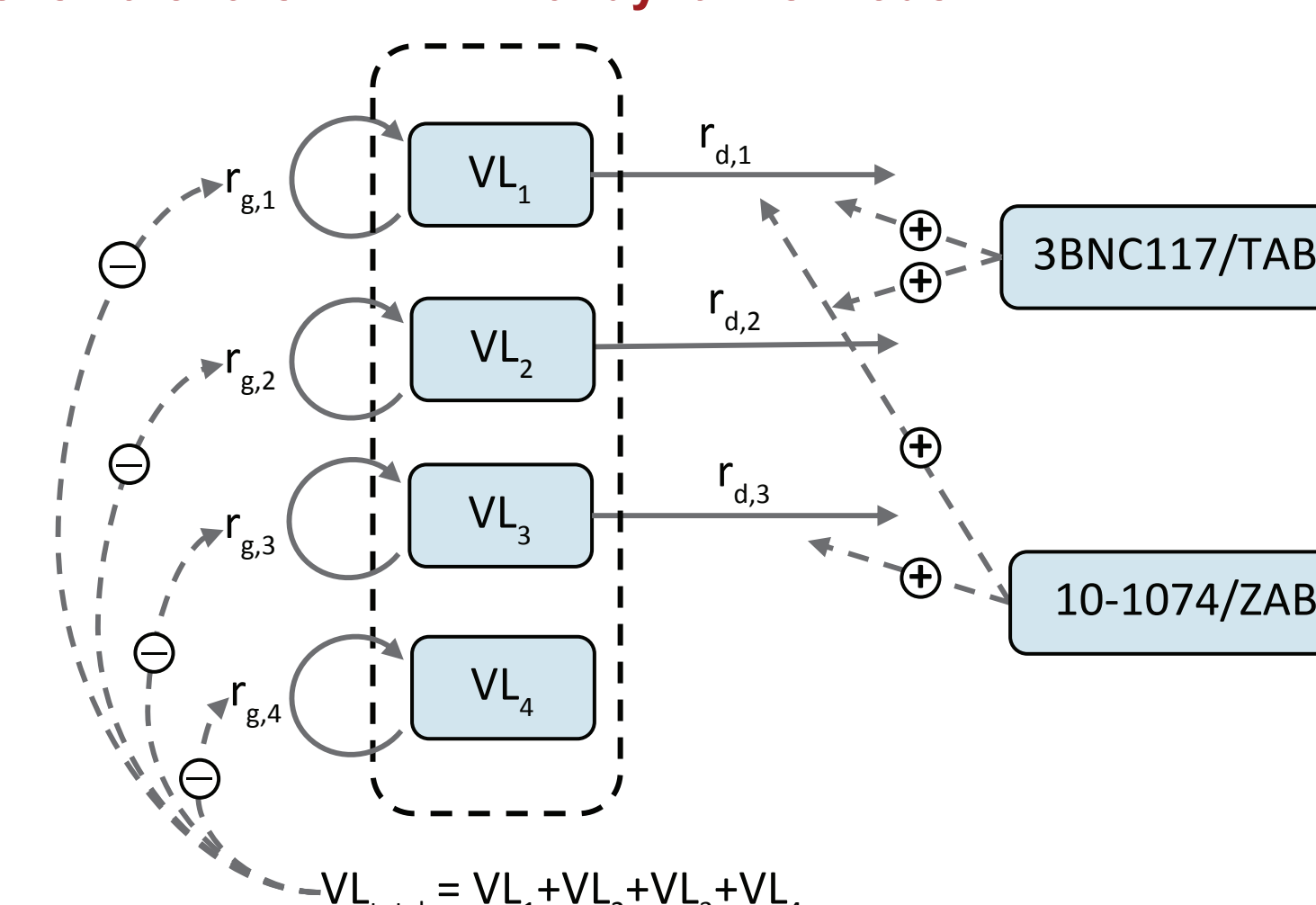
Figure 1. Schema of the PK-PD viral dynamic model
